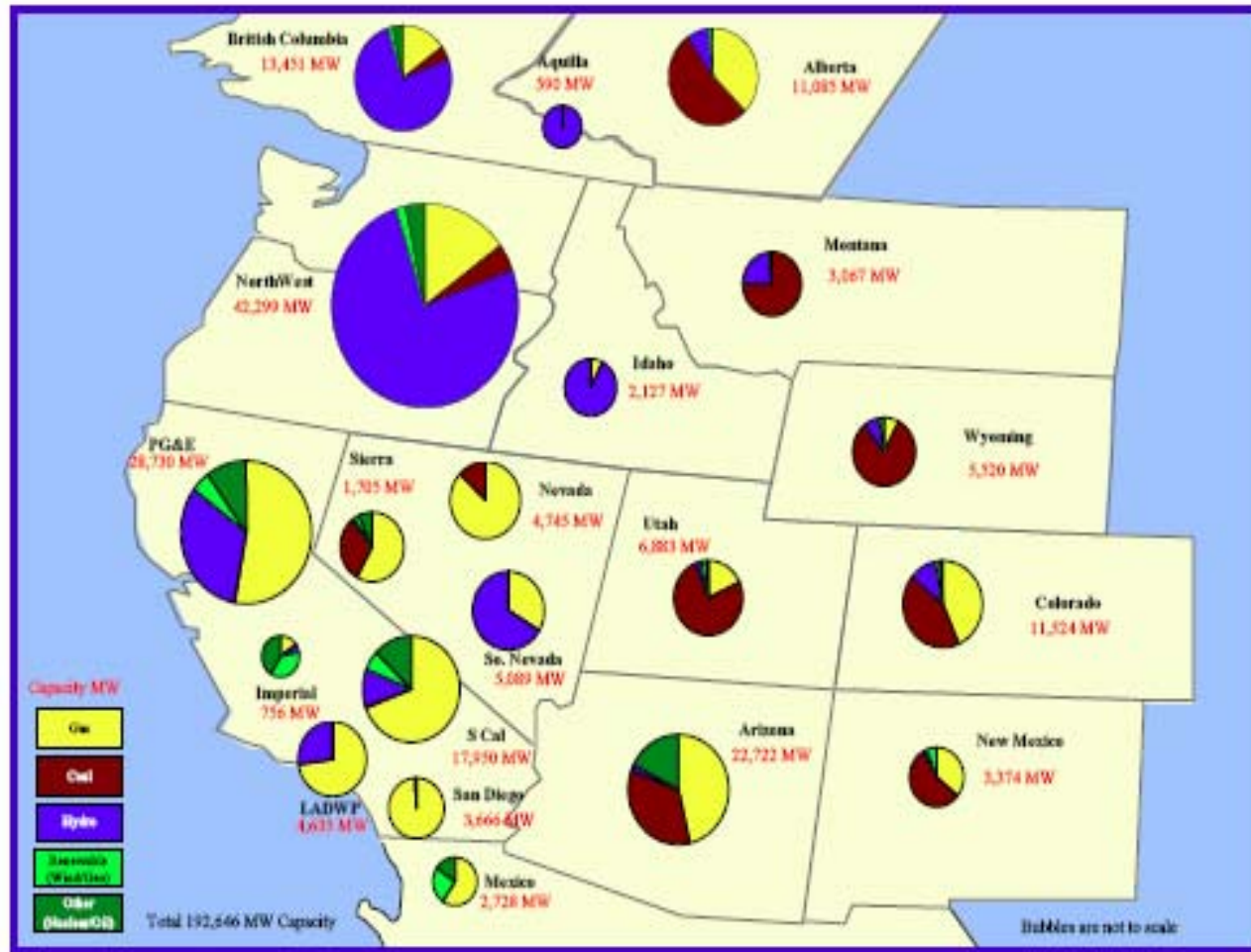
Figure 1- 2: 2008 forecasted generating resource capacity in the Western Interconnection by fuel type
