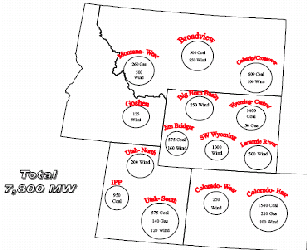
Figure E-3: Generation Additions Assumed in Recommendation 2
